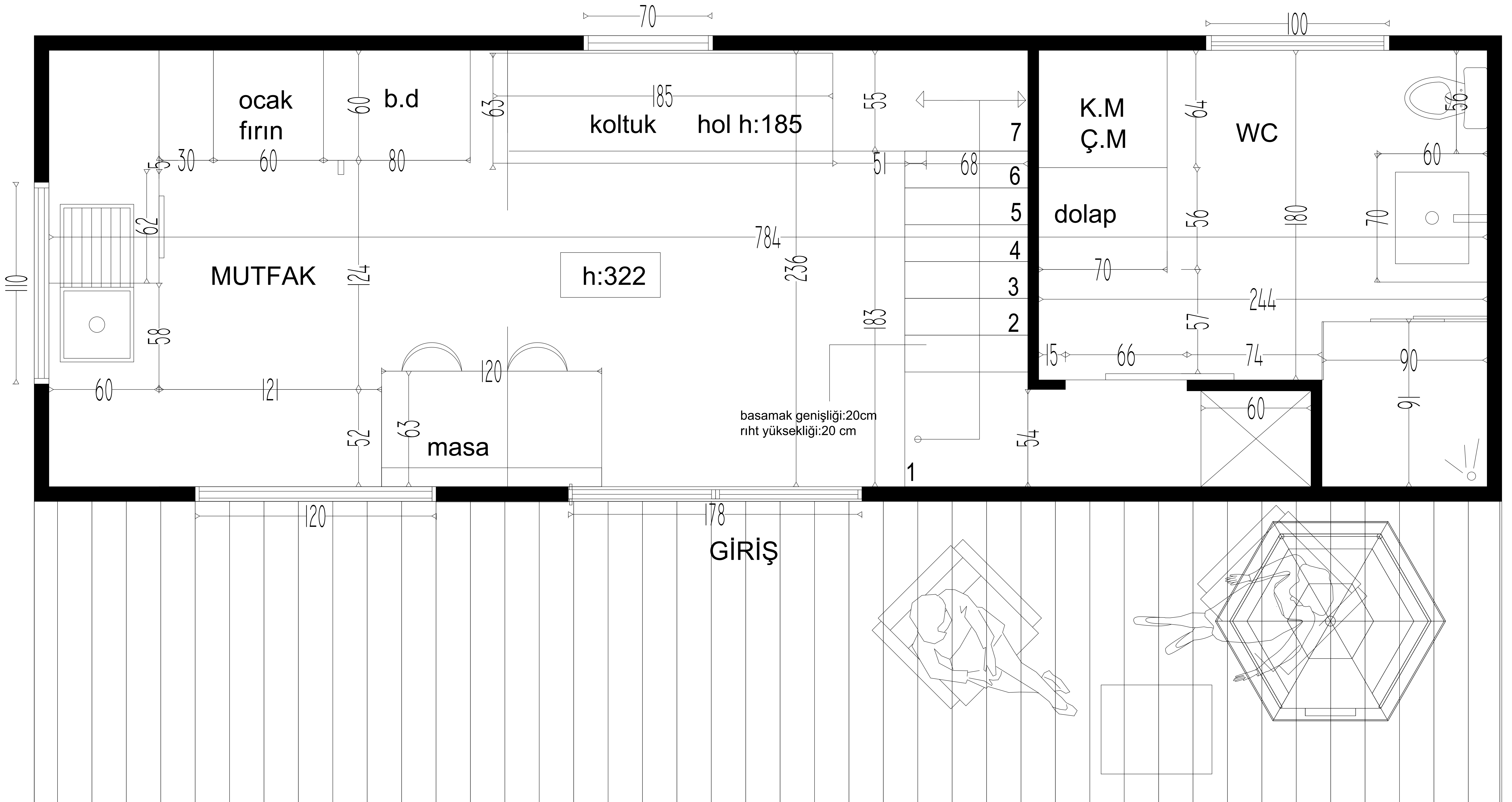
TINY HOUSE ALT KAT PLANI
